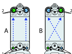
Figuur 6. Dubbel circuit: A is parallelle stroming; B is diagonale stroming.
