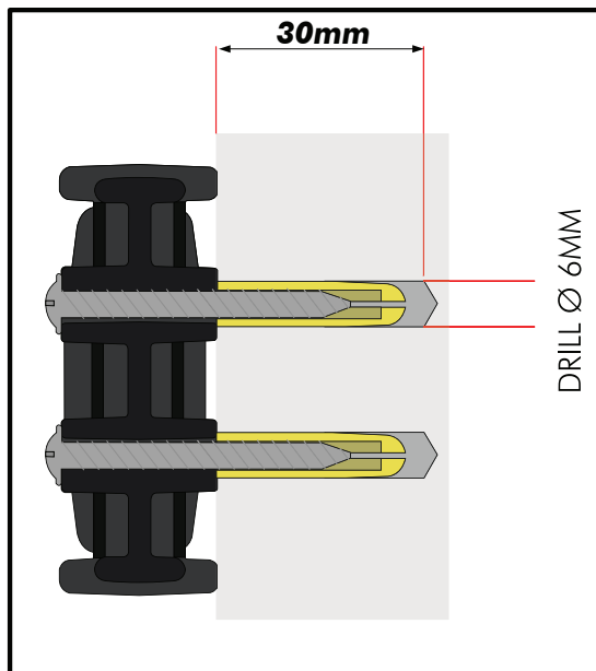
SECURING THE MOUNTING FEET
