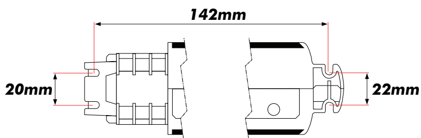
WITHOUT MOUNTING FEET
