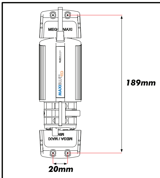
PUMP FITTED WITH MOUNTING FEET
