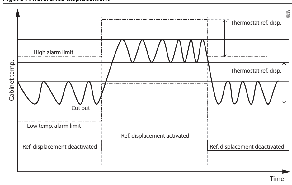
Figure 7: Reference displacement
