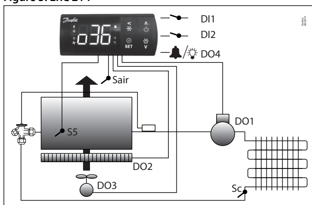
Figure 3: ERC 214
