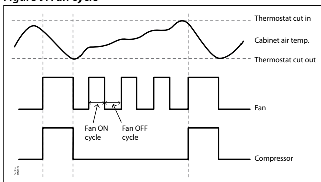
Figure 9: Fan cycle
