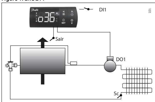
Figure 1: ERC 211
