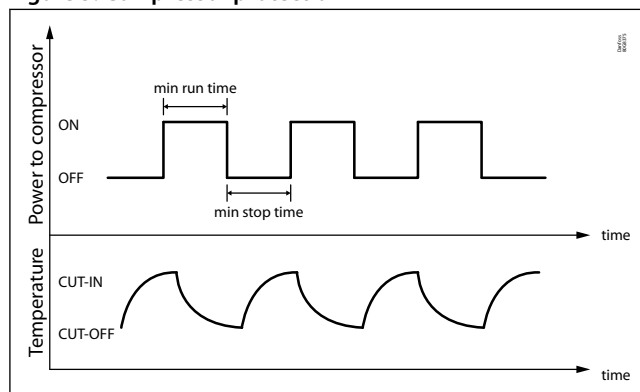
Figure 5: Compressor protection
