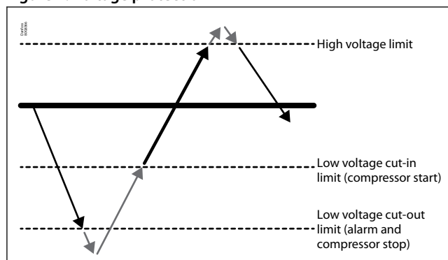
Figure 4: Voltage protection
