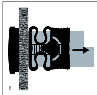
Figure 17: Dismounting
