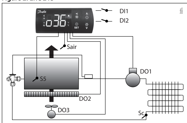
Figure 2: ERC 213
